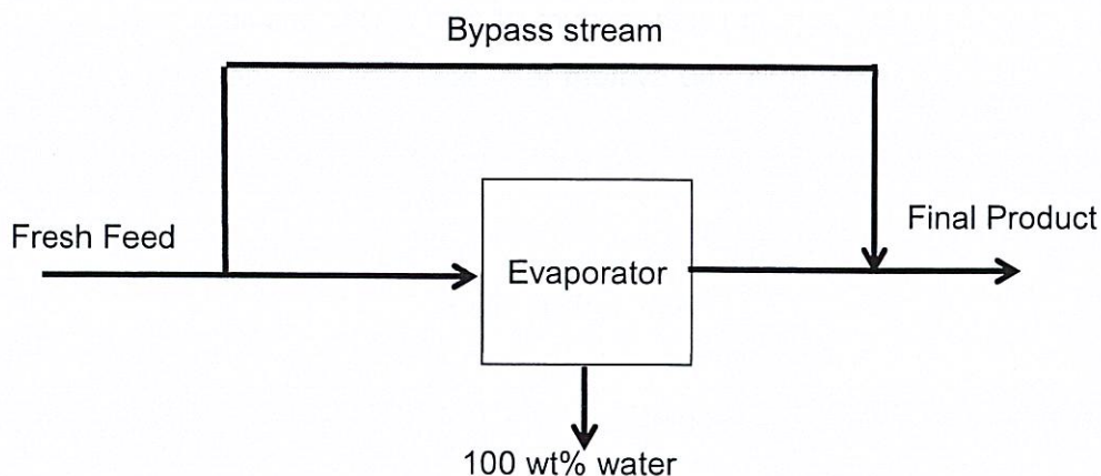
Figure 1: Evaporation Process
