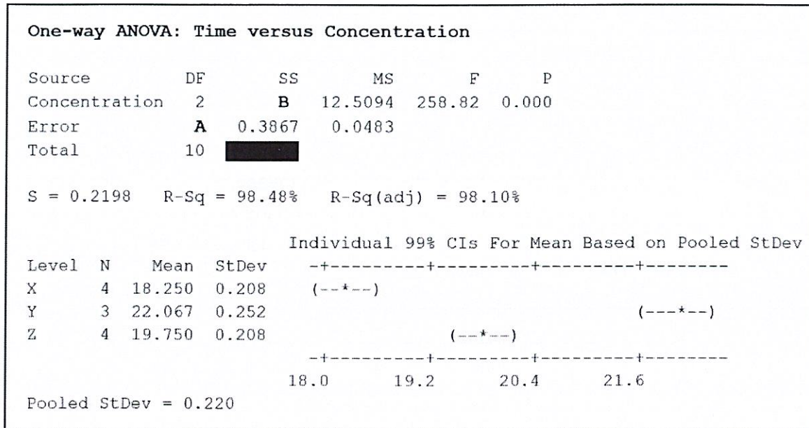
Figure 2: MINITAB output
