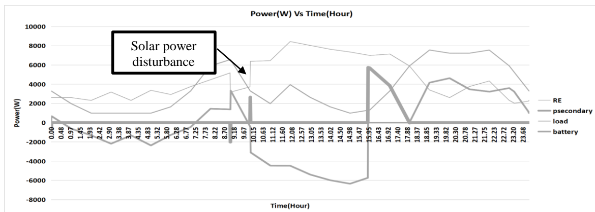
Figure 12. RESs and DESs power after a sudden decrease in solar power plant
