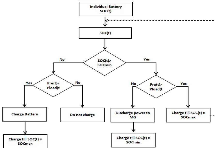
Figure 2. Flowchart of the Proposed M-G
