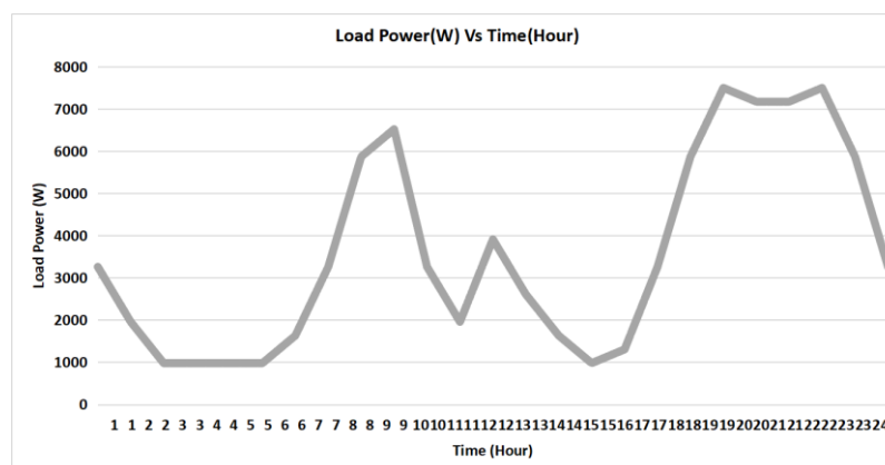
Figure 5. Load demand at micro-grid
