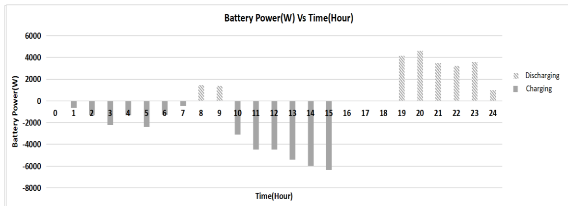
Figure 7. Battery Power on charging and discharging modes at the micro-grid
