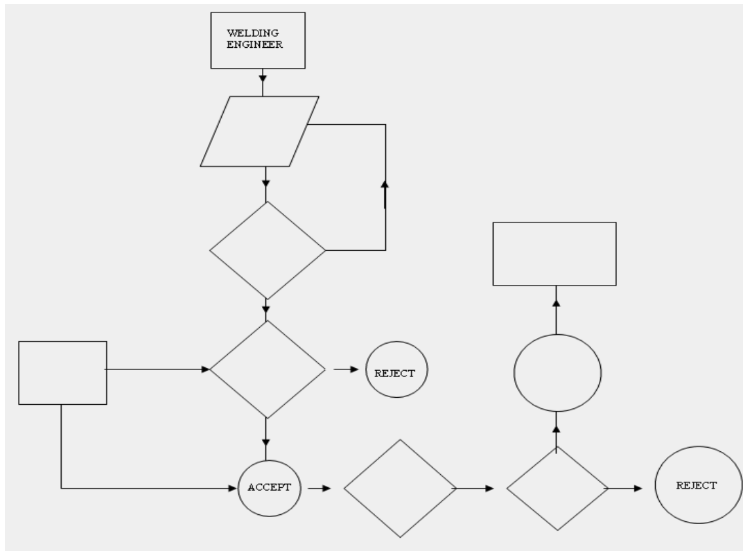
0: WELDING PROCEDURE QUALIFICATION FLOWCHART
