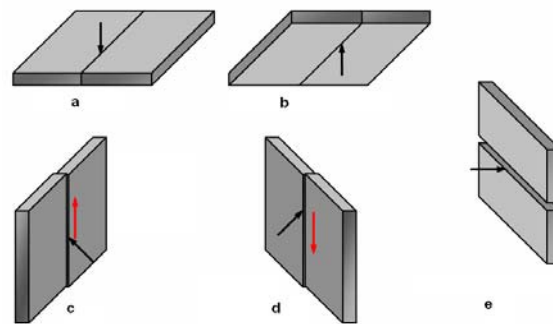
Figure 1.0 .welding position ( ISO 6947)
